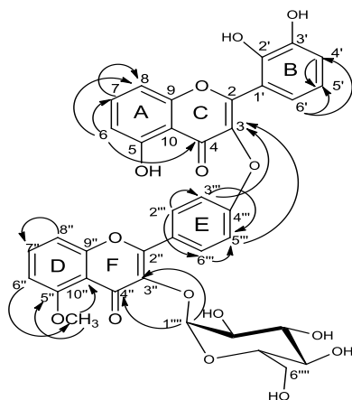
Figure 3. Key HMBC of compound 3
