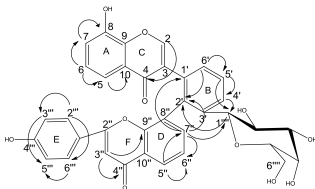
Figure 2. Key HMBC of compound 2
