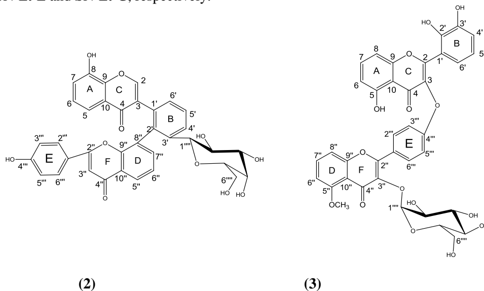
Figure 1. Structures of new compounds ( 2 and 3 ) from Solanum nigrum L.
