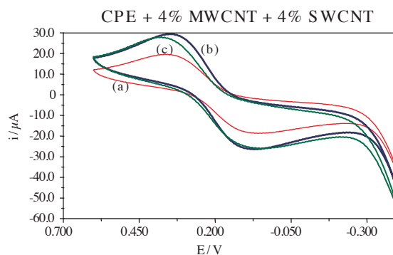
Figure 3. The cyclic voltammograms of 2 mM ferricyanide with (a) CPE, (b) 4% MWCNT-CPE, (c) 4% SWCNT-CPE; all other conditions as in Figure 2.
