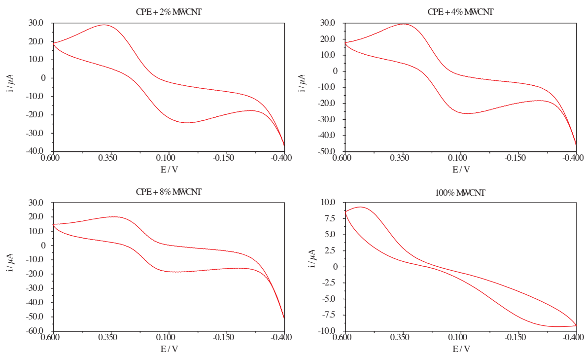
Figure 1. The effect of MWCNT amount on cyclic voltammograms of 2 mM ferricyanide, in the potential range of 600 to -400 mV, scan rate 100 mV/s, 50 mM phosphate buffer supporting electrolyte pH 7.
