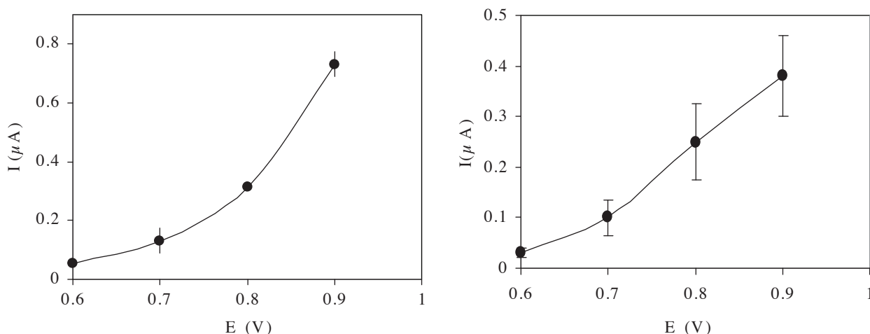
Figure 4. The effect of operating potential on current values for 1 mM \text{H}_2\text{O}_2 at (A) 4% MWCNT modified, (B) 4% SWCNT modified CPE.
